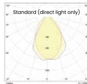
Light Distribution Beam Angle 70°
