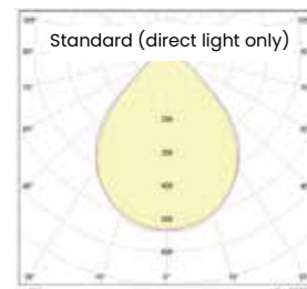
Light Distribution Beam Angle 100°
