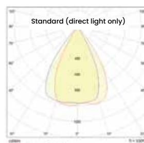
Light Distribution Beam Angle 90°
