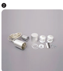
R75-08 Astrowave vertical suspension kit
