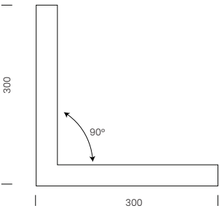
Dimensions (mm)
